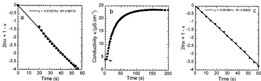
Figure 2. Oxidative addition of cis -1 (0.1 M) to the palladium(0) species generated in situ from Pd(dba) 2 (1 mM) and PPh 3 (2 mM) in DMF at 15 °C. a) As monitored by UV spectroscopy: variation of 2\ln x + 1 - x vs. time [ x = (D - D_{\text{lim}})/(D_0 - D_{\text{lim}}) ] ( D : absorbance of [Pd 0 (dba)(PPh 3 ) 2 ] at time t ; D_0 : initial absorbance of [Pd 0 (dba)(PPh 3 ) 2 ]; D_{\text{lim}} : absorbance at infinite time). b) Kinetics of the formation of the cationic complex 2^+\text{EtOCO}_2^- generated in the oxidative addition under the same conditions as in part a of this figure, as monitored by conductivity measurements. c) Variation of 2\ln x + 1 - x vs. time [ x = (\kappa_{\text{lim}} - \kappa)/(\kappa_{\text{lim}} - \kappa_0) ] ( \kappa : conductivity of 2^+\text{EtOCO}_2^- at time t ; \kappa_0 : residual initial conductivity; \kappa_{\text{lim}} : final conductivity of 2^+\text{EtOCO}_2^- ).
