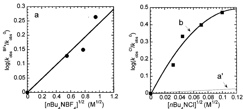
Figure 3. a) Effect of the ionic strength in the reaction of cis -1 (0.1 M) with the Pd 0 complex generated from Pd(dba) 2 (1 mM) and PPh 3 (2 mM) in DMF at 15 °C. Variation of \log(k_{\text{obs}}^{\text{BF}_4}/k_{\text{obs}}^0) vs. the square root of n Bu 4 NBF 4 concentration. b) Specific effect of chloride ions in the reaction of cis -1 (0.1 M) with the Pd 0 complex generated from Pd(dba) 2 (1 mM) and PPh 3 (2 mM) in DMF at 15 °C. Variation of \log(k_{\text{obs}}^{\text{Cl}}/k_{\text{obs}}^0) vs. the square root of n Bu 4 NCl concentration. a') Theoretical effect of the ionic strength due to the presence of n Bu 4 NCl. The straight line in part a' of this figure has been rebuilt from the straight line of part a.
