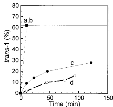
Figure 4. Effect of chloride ions on the kinetics of the isomerization of cis -1 to trans -1 induced by [Pd 0 (PPh 3 ) 4 ] in CDCl 3 . a) cis -1 + [Pd 0 L 4 ] (20 mM/20 mM); b) cis -1 + [Pd 0 L 4 ] + Cl − (20 mM/20 mM/20 mM); c) cis -1 + [Pd 0 L 4 ] + Cl − (200 mM/20 mM/20 mM); d) cis -1 + [Pd 0 L 4 ] + Cl − (200 mM/20 mM/200 mM).
