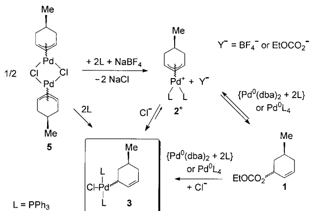
Scheme 16. For clarity, the stereochemistry of the complexes is not shown (see text and Scheme 8).
