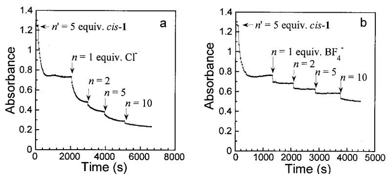
Figure 1. UV spectroscopy at 396 nm in DMF at 20 °C. a) Initial absorbance of [\text{Pd}^0(\text{dba})(\text{PPh}_3)_2] (1 mM) generated from \text{Pd}^0(\text{dba})_2 (1 mM) and \text{PPh}_3 (2 mM). The arrows indicate the addition of n' = 5 equiv. of cis -1 at t = 100 s and then successive additions of n equiv. of n\text{Bu}_4\text{NCl} . b) The same experiment as in part a of this figure but with addition of n\text{Bu}_4\text{NBF}_4 . In both cases, n is the total number of added equivalents.
